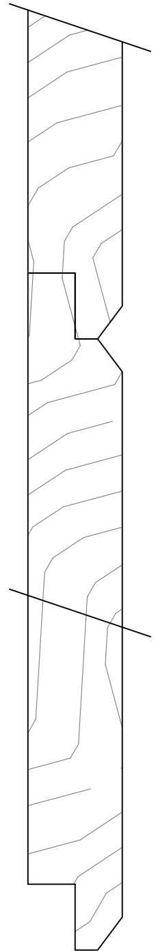
GCM121 2\frac{3}{32} X VARIES
