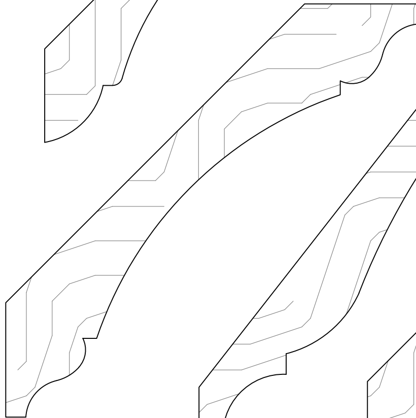
GCM599 Projection 4\frac{1}{4} Height 4\frac{1}{4} 1 X 6
