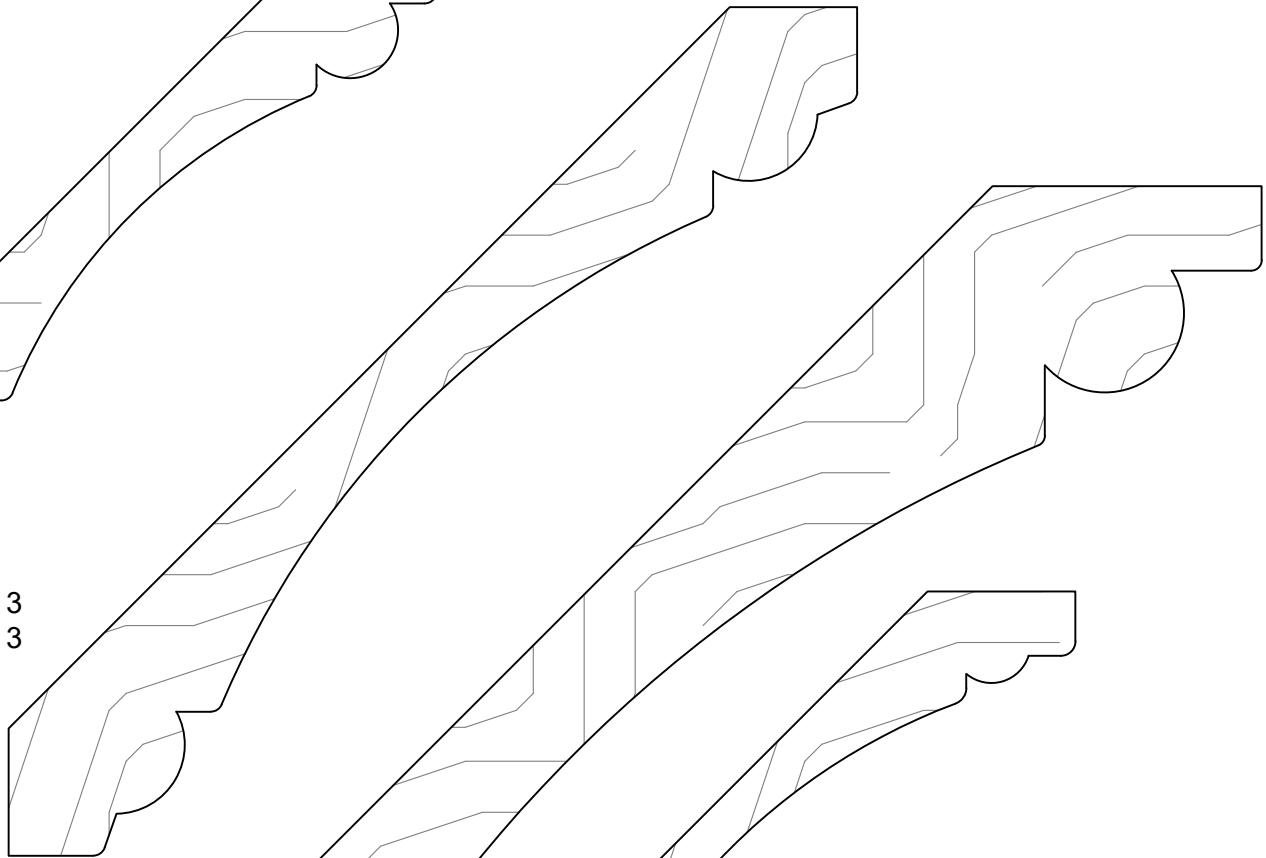
GCM335 Projection 4\frac{13}{32} Height 4\frac{13}{32} 1\frac{3}{16} \times 6\frac{1}{4}
