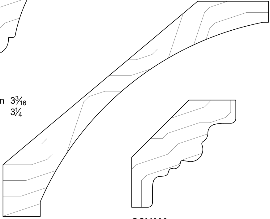
GCM632 Projection 1\frac{13}{16} Height 1\frac{3}{4} \frac{13}{16} X 2\frac{1}{2}
