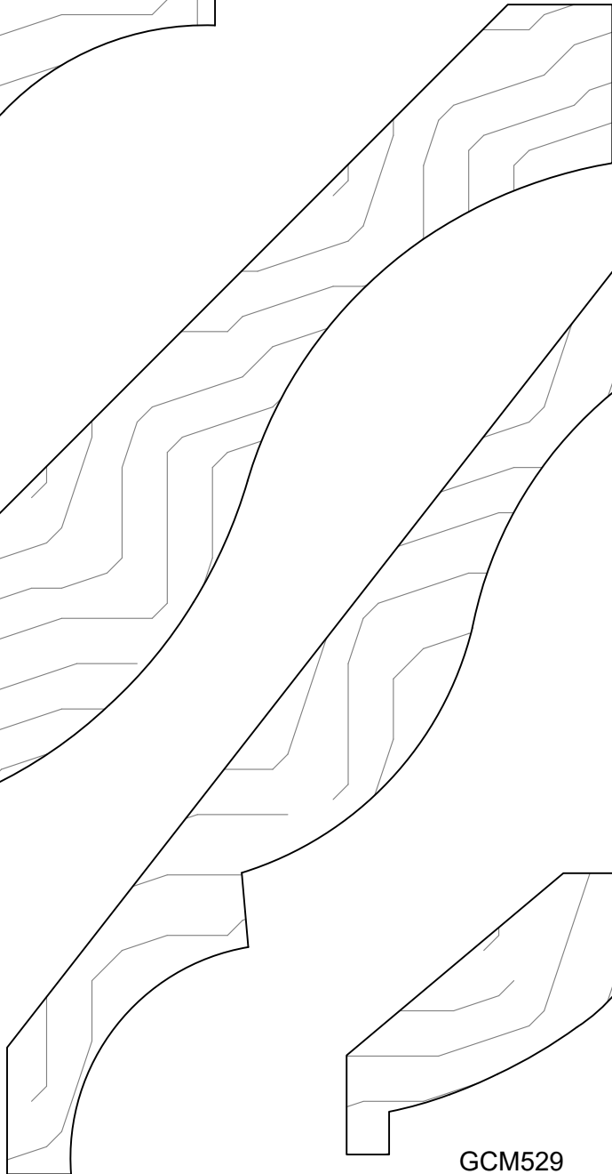
GCM44681 Projection 4\frac{1}{4} Height 4\frac{7}{16} 1\frac{3}{16} \times 6\frac{7}{8}
