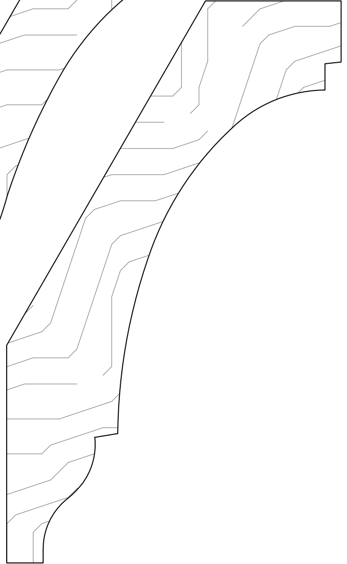
GCM35 Projection 3\frac{3}{8} Height 5\frac{1}{16} 1\frac{1}{2} \times 6\frac{5}{8}
