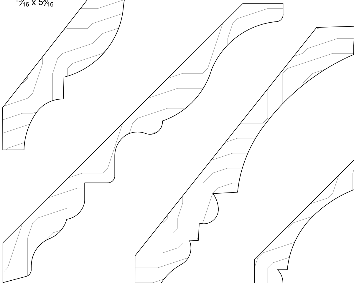
GCM601 Projection 5 Height 5 \frac{3}{4} \times 7
