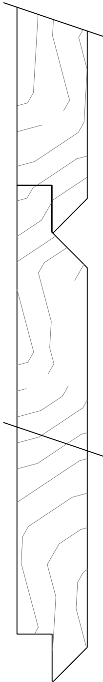
GCM3501 \frac{3}{4} x 7\frac{3}{4} 7 \frac{1}{4} " FACE
