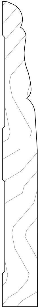
GCM664 5/8 x 5 1/2"
