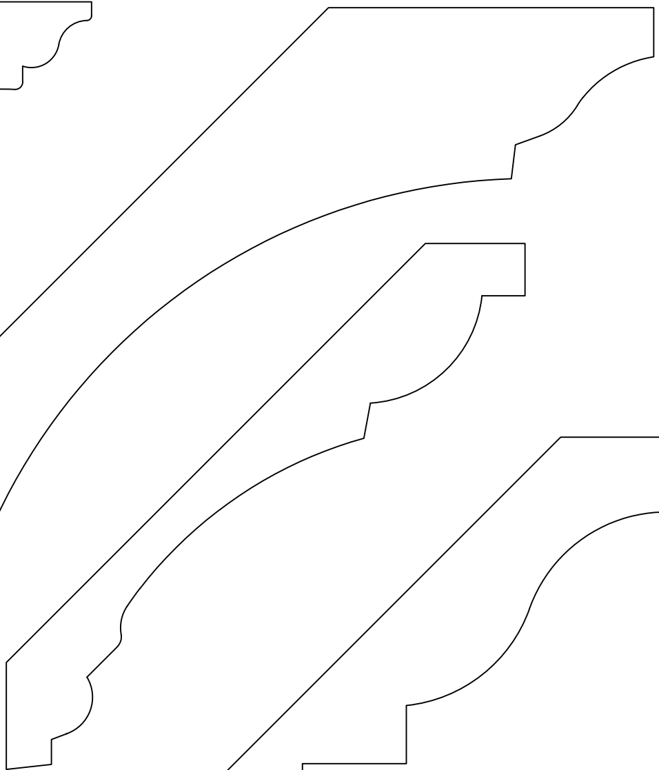
GCM642 Projection 3\frac{15}{16} Height 3\frac{15}{16} 1\frac{3}{16} X 5\frac{5}{8}
