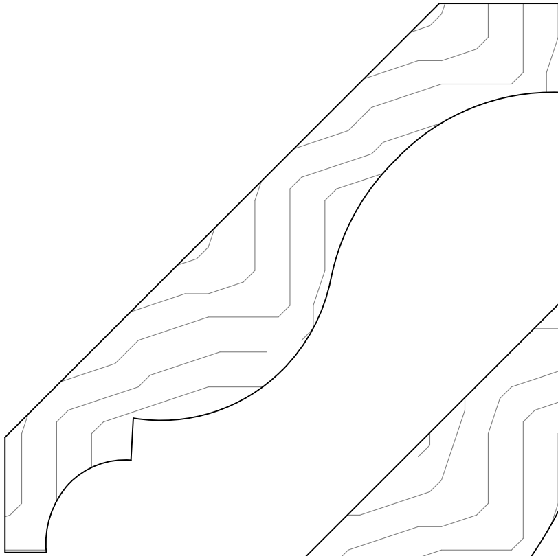
GCM1010 Projection 4\frac{3}{16} Height 4\frac{3}{16} 1\frac{1}{8} \times 5\frac{15}{16}
