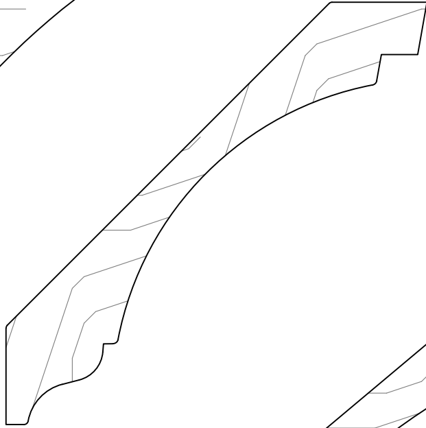
GCM626 Projection 3\frac{3}{16} Height 3\frac{1}{4} \frac{3}{4} X 4\frac{1}{2}
