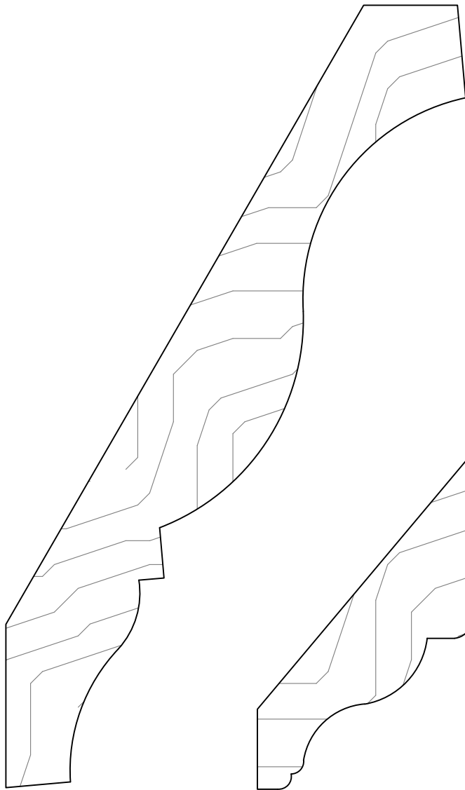
GCM1149 Projection 3\frac{3}{8} Height 5\frac{13}{16} 1 \times 6\frac{1}{16}
