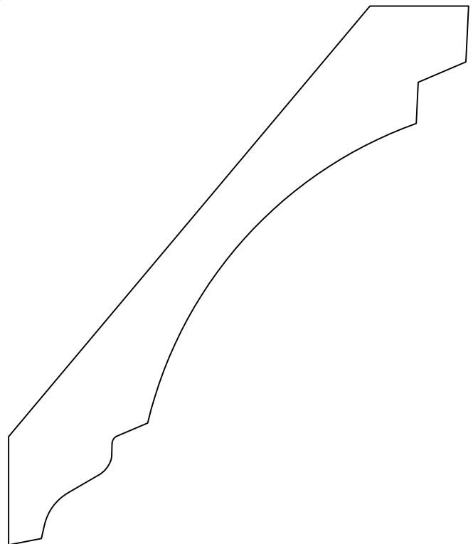
GCM653 Projection 3\frac{3}{8} Height 3\frac{15}{16} 1\frac{3}{16} \times 5\frac{3}{16}
