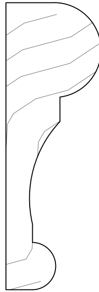
GCM7001 1 x 3
