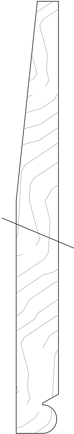
GCM145 3/4 x 9 1/4 7" FACE
