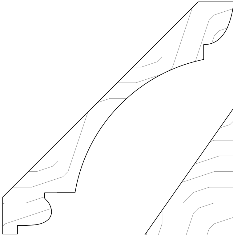
GCM80012 PROJECTION 3\frac{15}{16} " HEIGHT 3\frac{15}{16} " 1\frac{3}{16} " x 5\frac{1}{2} "
