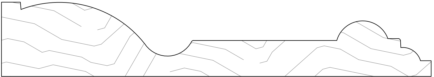
GCM1913 MOD 1¼ X 7¼"
