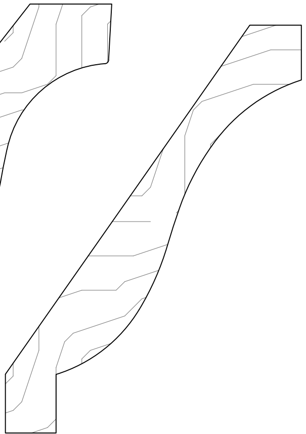
GCM576 Projection 3\frac{1}{16} " Height 4\frac{3}{16} " \frac{3}{4} \times 5\frac{3}{16} "
