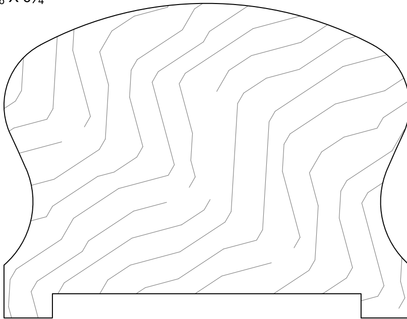
GCM5046 3 \frac{1}{4} X 4 \frac{3}{16}
