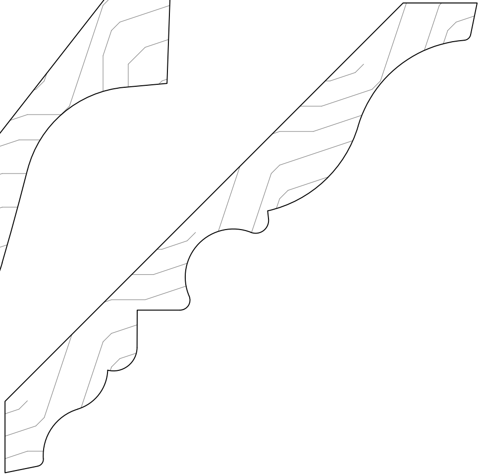
GCM634 Projection 4 \frac{15}{16} Height 4 \frac{15}{16} \frac{3}{4} \times 7
