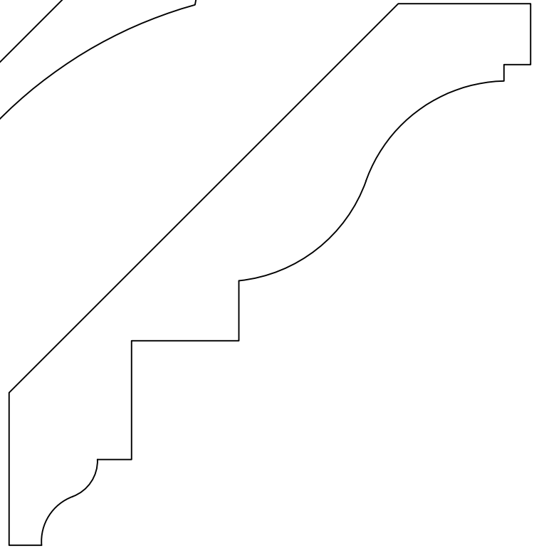
GCM643 Projection 3\frac{13}{16} Height 3\frac{15}{16} 1 X 5\frac{1}{2}
