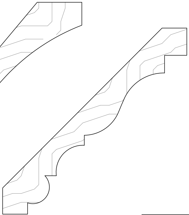
GCM553 PROJECTION 3 \frac{1}{16} " HEIGHT 3 \frac{1}{16} " \frac{3}{4} X 5 \frac{1}{4} "
