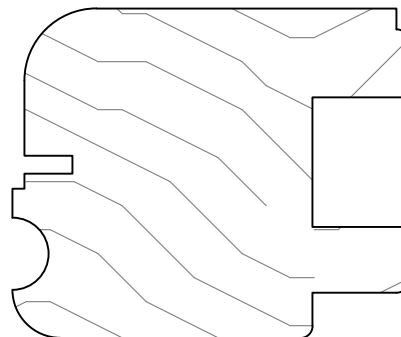
GCM6006 1 3/4 x 2 1/16
