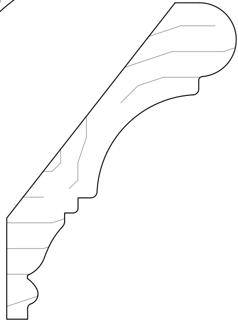
GCM554 PROJECTION 2\frac{3}{8} " HEIGHT 3\frac{1}{4} " \frac{13}{16} X 3\frac{7}{8} "
