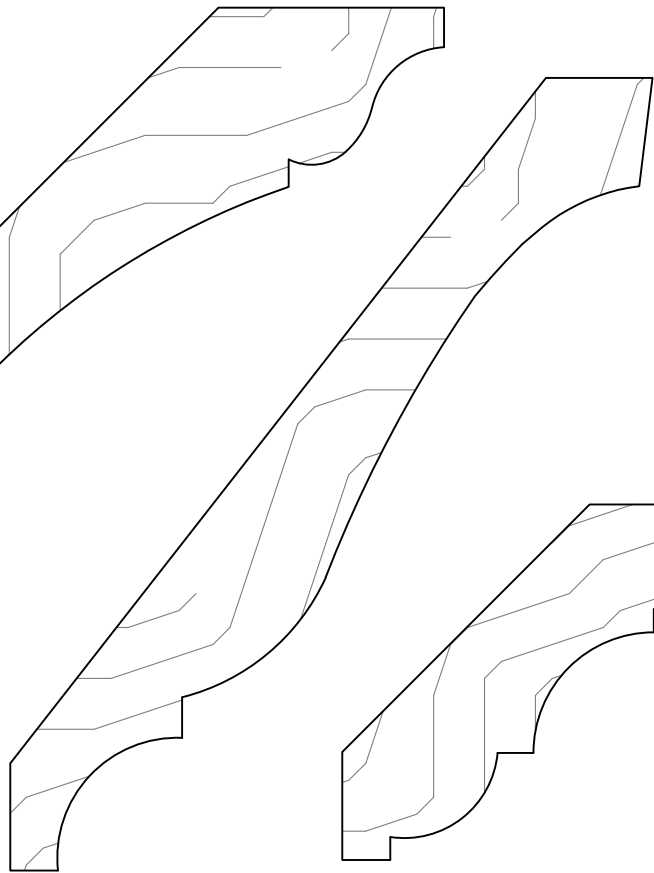
GCM1045 Projection 1\frac{13}{16} Height 2 \frac{3}{4} \times 2\frac{5}{8}
