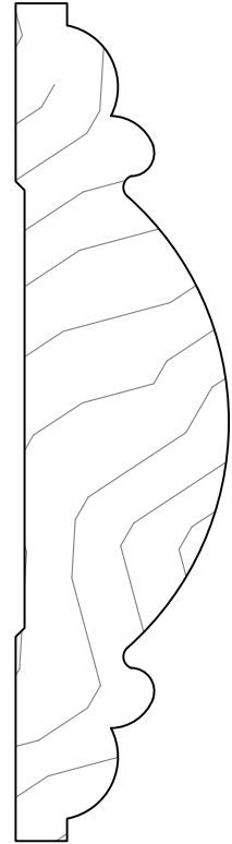
GCM395 1 x 4
