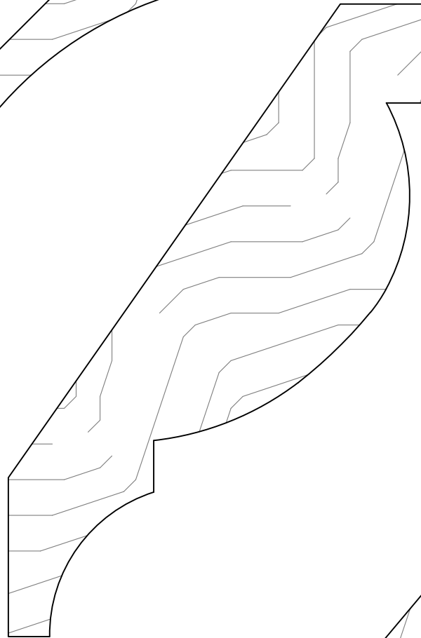
GCM80019 PROJECTION 3\frac{1}{16} " HEIGHT 4\frac{1}{16} " 1\frac{1}{2} " x 5\frac{5}{8} "
