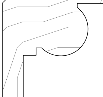
GCM24 Projection 5\frac{1}{2} " Height 5\frac{1}{2} " 1\frac{1}{2} X 7\frac{3}{4}
