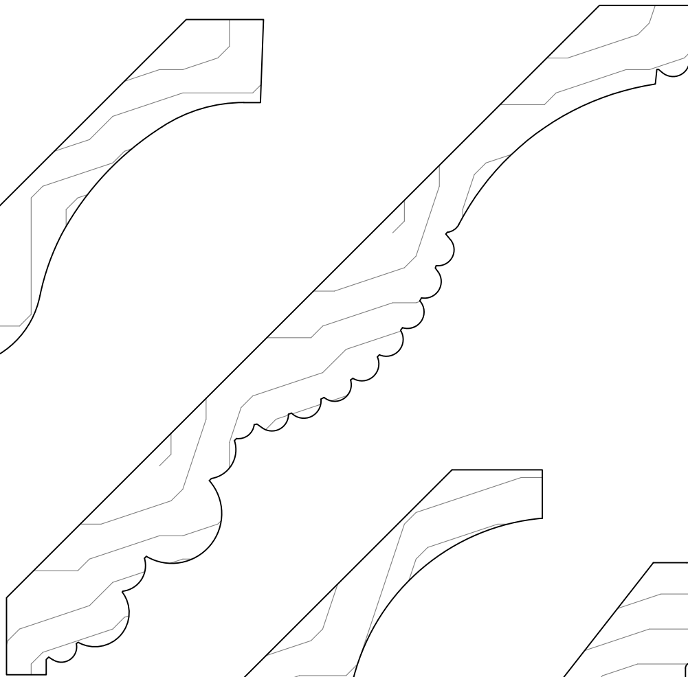
GCM522 Projection 5" Height 5" \frac{3}{4} X 7\frac{1}{4} "
